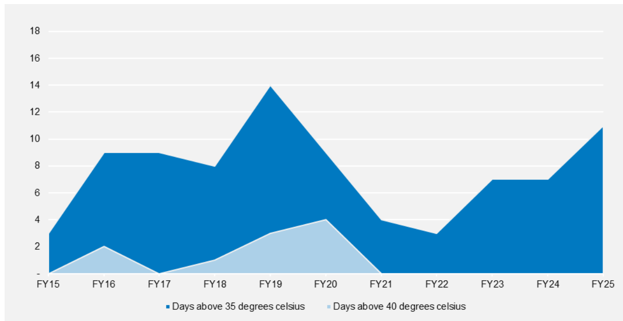
FIGURE 1.1 INNER MELBOURNE HISTORICAL TEMPERATURE: HOT DAYS
